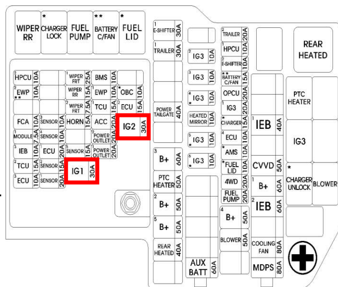
Engine room fuse box
